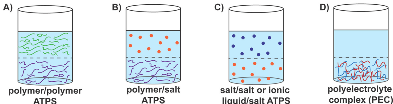
Fig. 1 An overview of various aqueous two-phase systems (ATPS) comprising water–water interfaces. (A) Segregative polymer/polymer ATPS, comprising immiscible solutions of incompatible polymers (depicted as green and purple chains). A common example is aqueous poly(ethylene glycol) (PEG)/dextran solution. (B) Segregative polymer/salt ATPS, comprising immiscible solutions of incompatible polymer and salt (depicted as purple chain and orange dots, respectively). A common example is aqueous solution of PEG and magnesium sulfate. (C) Segregative salt/salt ATPS, or ionic liquid/salt ATPS, comprising immiscible solutions of incompatible salts (depicted as orange and navy dots). Aqueous solution of lithium chloride and lithium bis(trifluoromethanesulfonyl)imide is an example of such a system. (D) Associative ATPS, comprising polyelectrolyte complexes (PECs), which are composed of a complex phase of polyanions (depicted in blue chains) and polycations (depicted in red chains) in equilibrium with the polymer-lean supernatant phase. Common examples of polyanions include poly(acrylic acid), poly(styrene sulfonate), succinyl amylose, poly(glutamic acid), poly(aspartic acid), and DNA. Common examples of polycations include poly(diallyldimethylammonium)chloride, poly(allylamine), poly(4-vinylridine) (P4VP), quaternized amylose, poly(lysine), and poly(arginine).
