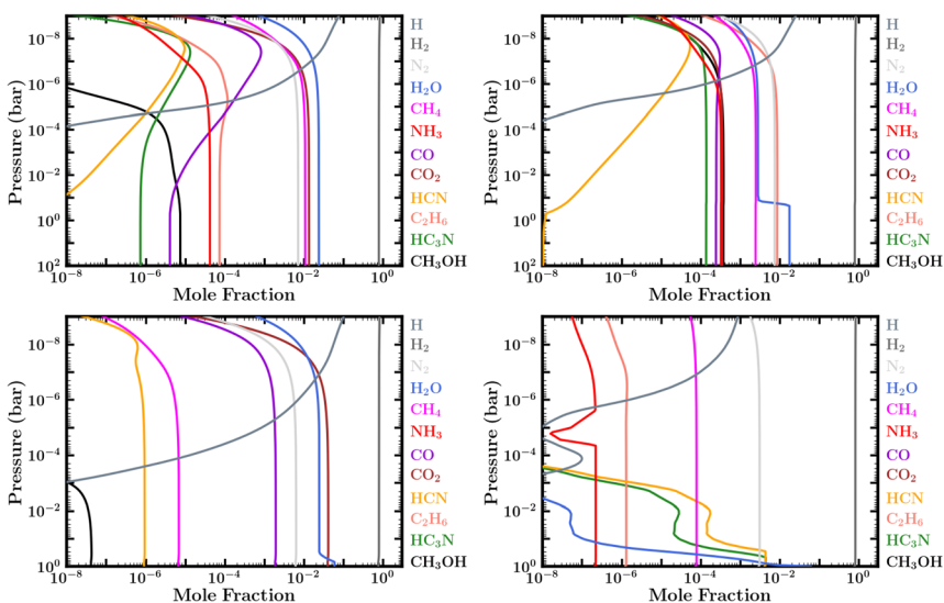
Fig. 3 Fully evolved (steady state) volume mixing-ratio profiles of prominent volatile species with zero-flux boundary conditions (inactive surface) for a 100× solar composition atmosphere and surface pressure of (top) 100 bar and (bottom) 1 bar: (top left) for the PT1 temperature profile in Fig. 2, corresponding to case 1 in Table 1; (top right) for the PT3 temperature profile, corresponding to case 3; (bottom left) for the PT1 temperature profile, corresponding to case 4; (bottom right) for the PT4 temperature profile, corresponding to case 6. Note that the sharp decline in \text{H}_2\text{O} , \text{HCN} , \text{HC}_3\text{N} , and \text{NH}_3 with altitude in case 6 is due to condensation.
