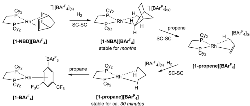
Scheme 1 Synthesis of \sigma -alkane complexes via single crystal-to-single crystal (SC–SC) transformations: (a) [1-NBA][Bar^F_4] by hydrogenation of [1-NBD][Bar^F_4] ; (b) [1-propane][Bar^F_4] from [1-NBA][Bar^F_4] via sequential NBA/propene substitution and hydrogenation.
