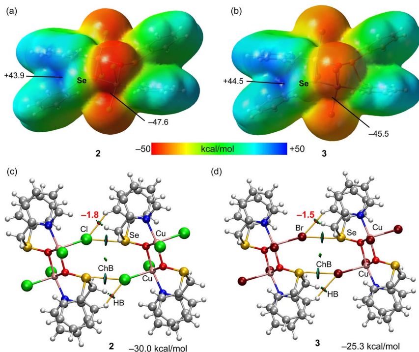
Fig. 3 (a and b) MEP surfaces of compounds 2 and 3 with indication of the MEP maximum and minimum. Energies in kcal mol −1 . (c and d) QTAIM (bond critical points in red and bond paths as orange lines) and NCIPLOT (RDG = 0.4, density cut-off = 0.04 a.u., color scale \pm 0.04 a.u.) representation for compounds 2 and 3 . Only intermolecular interactions are represented. The association energies in kcal mol −1 of the hydrogen bonds derived from V_r are given in red adjacent to the bond CP.
