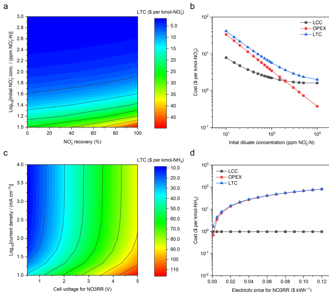
Fig. 5 Techno-economic analysis of upcycling \text{NO}_3^- -N from dilute waste streams. (a) The contour map for the LTC of \text{NO}_3^- -N concentration by electrodialysis with respect to the initial \text{NO}_3^- concentration in the diluate and the designed \text{NO}_3^- recovery from the diluate ( \$0.07 \text{ kW h}^{-1} of electricity cost). (b) LTC, OPEX, and LCC along with the initial diluate concentration ( \$0.07 \text{ kW h}^{-1} of electricity price and 80% of designed \text{NO}_3^- recovery). Based on a typical medium-size commercial electrodialysis system (40 cm \times 160 cm for each electrodialysis pair, and 250 electrodialysis pairs in total), the LCC was calculated via the standard capital recovery method, assuming 40 years of service time, 42 19% as the cost ratio of maintenance to the system, 3% of annual discount rate, 31 83.3% of capacity factor, and 90% of coulombic efficiency. (c) The contour map for the LTC of \text{NH}_3 production by NO3RR in MFAEL with respect to the electrolytic current density and cell voltage ( \$0.07 \text{ kW h}^{-1} of electricity price). (d) The impact of electricity price on the LTC and OPEX of the NO3RR (2.7 V of cell voltage and 250 \text{ mA cm}^{-2} of current density). Capital cost analysis was performed based on a customized medium-size MFAEL reactor with 100 L electrolyte capacity with the total electrode area of 3.36 \text{ m}^2 . The cost of all identified materials and ancillary/auxiliary parts/components was estimated to be \$1164 per system. Considering all unidentified parts (10%) and all other associated costs, 30 the total capital cost of this electrolyzer system was projected to be \$3121 per system. Other assumptions and methodologies are discussed in the ESI†.
