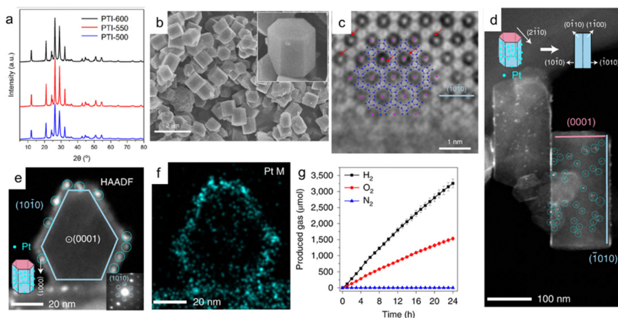
Fig. 8 (a) PXRD patterns of PTI samples. (b) SEM image showing the well-developed prism-like shape of \text{PTI}/\text{Li}^+\text{Cl}^- crystals. The inset shows the expanded view of a crystal. (c) The AC-iDPC images of a typical \text{PTI}/\text{Li}^+\text{Cl}^- crystal aligned along the [0001] direction. The positions of C, N and Cl atoms are superimposed. Some typical Li ions are denoted by red arrows. (d) The HAADF-STEM image of a PTI crystal aligned to the [2\bar{1}10] direction. The inset shows a schematic illustration of the distribution of Pt particles on the surfaces of PTI crystals. The blue circles indicate the positions of Pt particles. (e) The HAADF-STEM image of a PTI crystal aligned close to the [0001] direction; the inset shows the diffraction pattern from the particle. Note that the side faces correspond to the \{10\bar{1}0\} facets. (f) EDS maps of the main Pt elements. (g) The accumulated amount of the gases produced by PTI-550 (evacuated at each hour after sampling). The error bars show standard deviation. Reproduced with permission from ref. 111 (Copyright 2020, Springer Nature).
