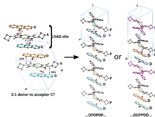
Fig. 1 Solid-state reaction in a 2 : 1 D to A CT co-crystal leading to two possible arrangements of product to donor arrangements if the reaction is cooperative. We found that SCSC reaction leads to the \cdots\{D\cdots P\}\cdots\{P\cdots D\}\cdots arrangement shown on the right. 23
