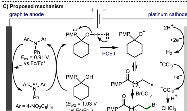
Scheme 6 Electrochemical deconstructive functionalisation of cycloalkanols via alkoxy radicals enabled by proton-coupled electron transfer (Morrill).
