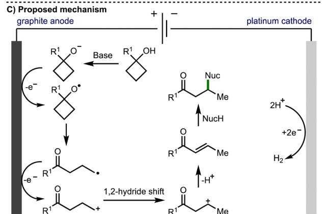
Scheme 7 Electrochemical synthesis of \beta -functionalised ketones via ring opening of cycloalkanols (Guo and Xia).
