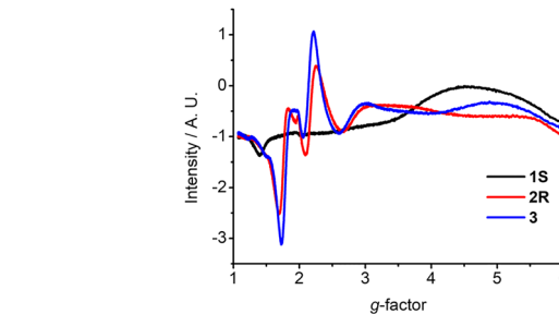
Fig. 2 EPR spectra of 1S , 2R , and 3 recorded in frozen acetonitrile at 100 K (concentration ~ 3.0 × 10 -3 M).
