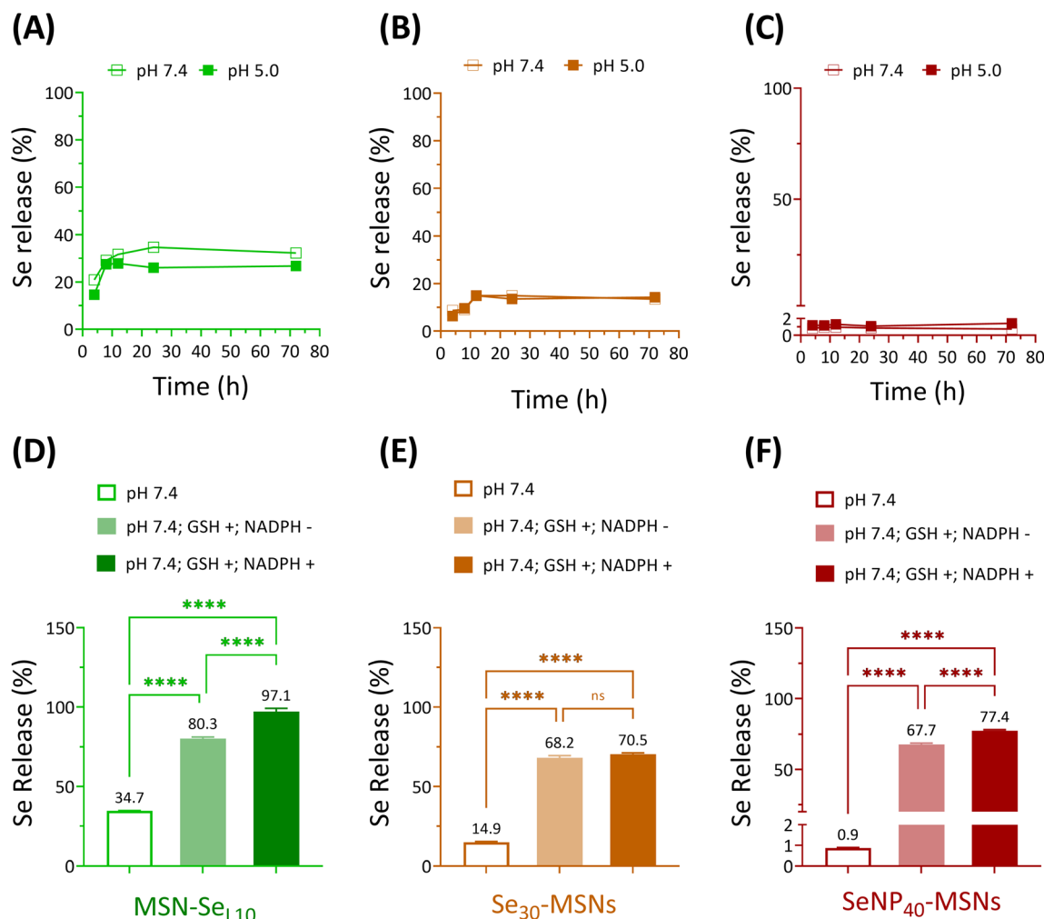
Fig. 3 Se release of (A) MSN-Se 10 , (B) Se 30 -MSNs and (C) SeNP 40 -MSNs in pH 7.4 and pH 5.0 at 4, 8, 12, 24, and 72 h incubation. Se release profiles of (D) MSN-Se 10 , (E) Se 30 -MSNs and (F) SeNP 40 -MSNs after 24 h incubation in the absence/presence of GSH (10 mM) and NADPH (1.0 mM) at neutral conditions. n = 3 . * represents p -values of significant differences compared to the controls. (*: p < 0.05 ; **: p < 0.005 ; ***: p < 0.001 ; ****: p < 0.0001 ).
