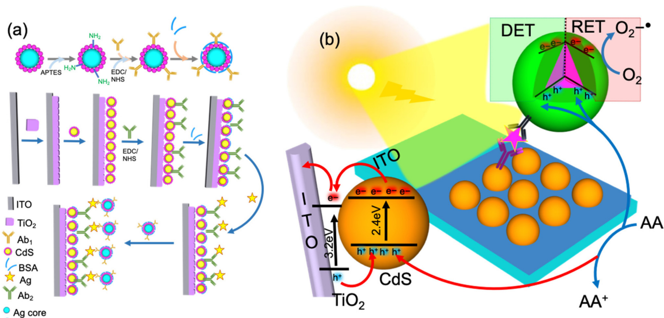
Fig. 5 The schematic illustration of: (a) the surface functionalization of an ITO/TiO 2 /CdS photoelectrochemical immunosensor and sandwich assay with Ag@Cu 2 O submicron particles for the detection of cardiac troponin, and (b) a PEC sensor showing the electron transport mechanism from CdS-sensitized TiO 2 nanohybrid and Ag@Cu 2 O SPs. 80 Reprinted with permission from ref. 80 (copyright © 2018 Elsevier B.V).
