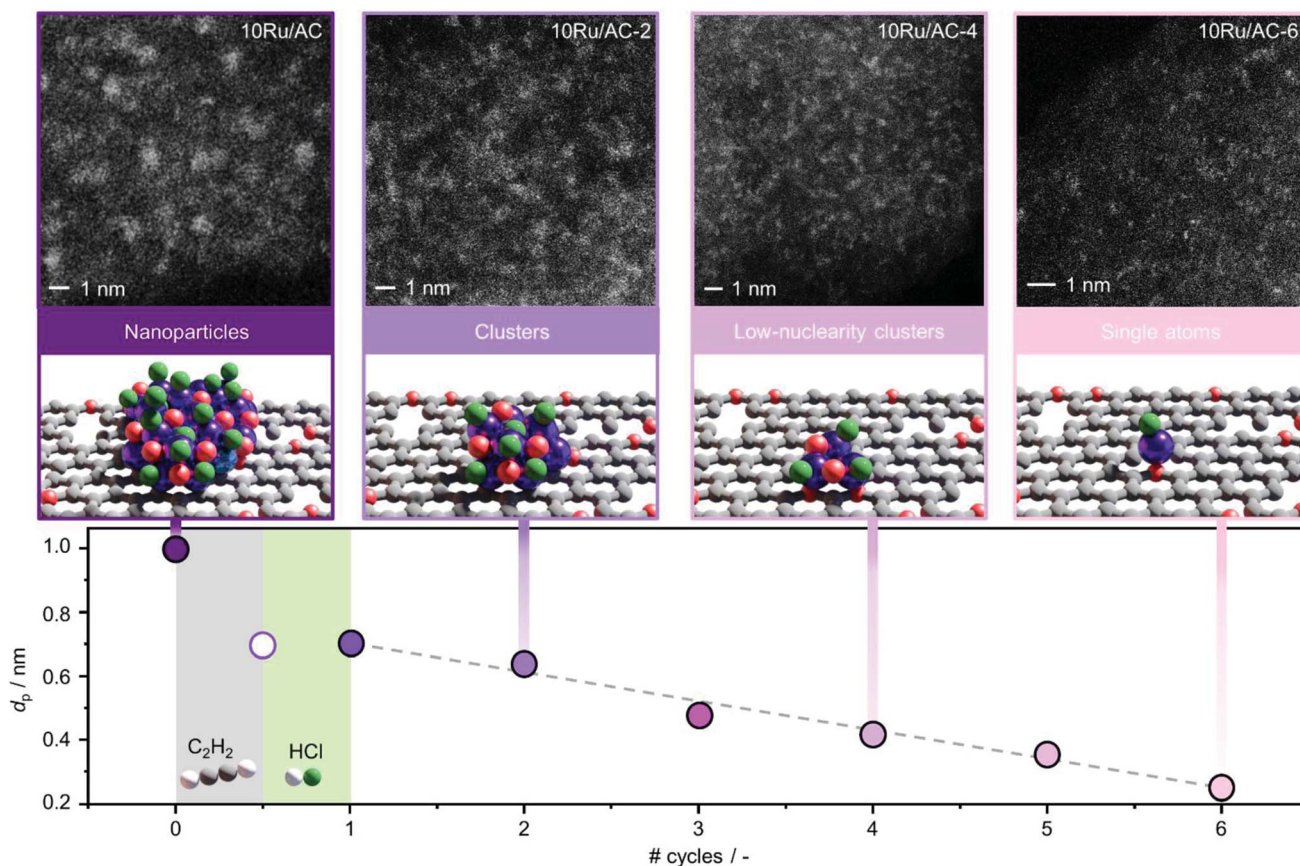
Fig. 2 Average metal particle size ( d_p ) of 10Ru/AC, in fresh and treated forms, as a function of the number of C 2 H 2 –HCl treatment cycles and HAADF-STEM images of selected samples, visualising the control over nuclearity enabled by the redispersion treatment. One cycle consists of exposure to C 2 H 2 atmosphere followed by exposure to HCl atmosphere, for 1 h each. Treatment conditions: W_{\text{cat}} = 0.1 g, F_T = 15 cm 3 STP min −1 , T = 473 K, C 2 H 2 treatment: 40 vol% C 2 H 2 , 44 vol% He, 16 vol% Ar, HCl treatment: 44 vol% HCl, 40 vol% He, 16 vol% Ar.
