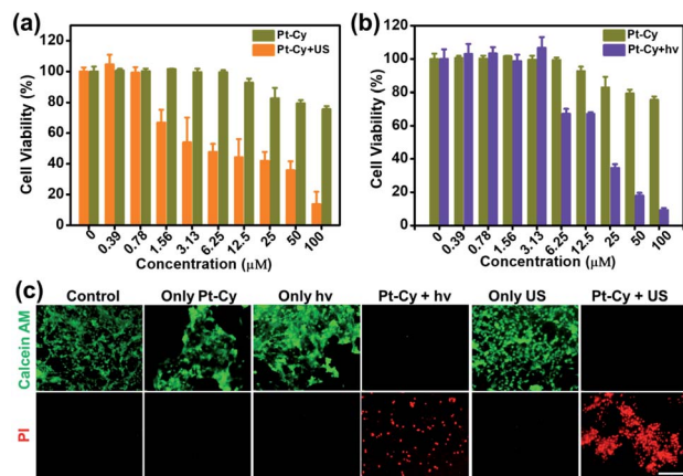
Fig. 2 The cell viabilities of 4T1 cells treated with different concentrations of Pt-Cy under (a) US irradiation (3.0 MHz, 0.3 \text{mW cm}^{-2} , 20 min) and (b) 465 nm light irradiation (10 \text{mW cm}^{-2} , 30 min). (c) Confocal microscopy images of the 4T1 cells treated with Pt-Cy (20 \mu\text{M} , 1 h) and then co-stained with calcein AM (4 \mu\text{M} , 0.5 h) and PI (6 \mu\text{M} , 0.5 h) after different treatments. Calcein AM: \lambda_{\text{ex}} = 458 \text{ nm} , \lambda_{\text{em}} = 540 \pm 30 \text{ nm} ; PI: \lambda_{\text{ex}} = 540 \text{ nm} , \lambda_{\text{em}} = 610 \pm 30 \text{ nm} ; scale bar: 100 \mu\text{m} .
