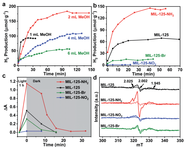
Fig. 2 (a) Dark photocatalytic hydrogen production activity of MIL-125 with different amounts of methanol at 25 °C. (b) Dark photocatalytic hydrogen production activity comparison of MIL-125 and MIL-125-X (X = NH 2 , NO 2 , Br) with 0.5 mL TEOA as a sacrificial agent at 25 °C. (c) Decay profiles of UV-Vis absorption at 530 nm (raw data in Fig. S18†). (d) ESR spectra (solid and dotted lines represent signals in the dark and when light is on, respectively) for MIL-125 and MIL-125-X (X = NH 2 , NO 2 , Br).
