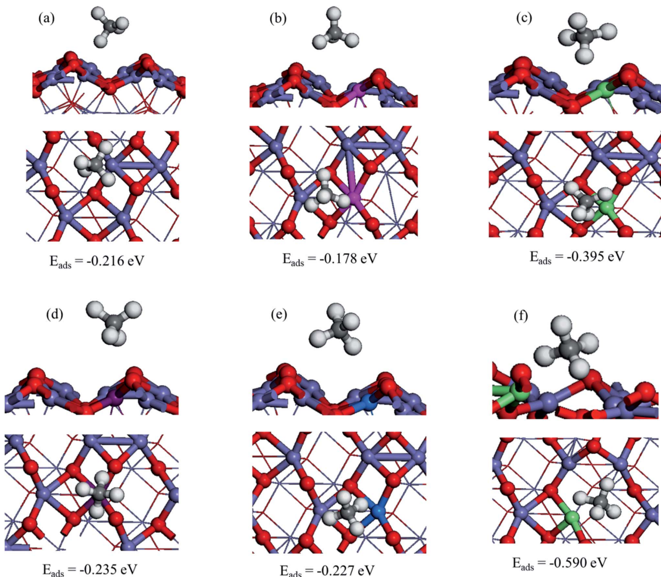
Fig. 2 Optimized structure of \text{CH}_4 adsorption on M/\alpha\text{-Fe}_2\text{O}_3(110) surfaces: (a) \alpha\text{-Fe}_2\text{O}_3(110) , (b) \text{Ag}/\alpha\text{-Fe}_2\text{O}_3(110) , (c) \text{Ir}/\alpha\text{-Fe}_2\text{O}_3(110) , (d) \text{Co}/\alpha\text{-Fe}_2\text{O}_3(110) , (e) \text{Cu}/\alpha\text{-Fe}_2\text{O}_3(110) , and (f) \text{Ir}/\alpha\text{-Fe}_2\text{O}_3(110)\text{-O}_V surfaces.
