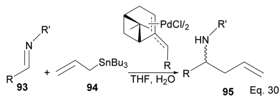
Scheme 26 (–)- \beta -Pinene-based \pi -allylpalladium assisted enantioselective allylation of imine.
