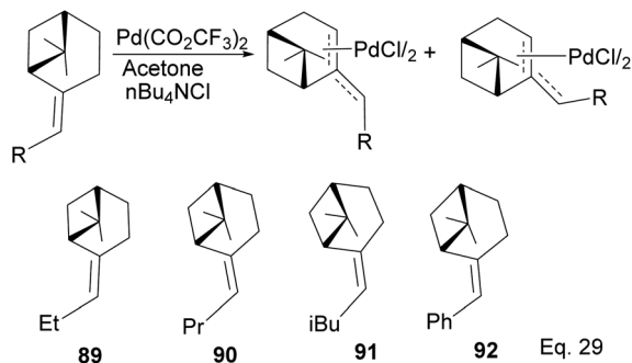
Scheme 25 (–)- \beta -Pinene-based \pi -allylpalladium catalyst used in allylation of imines.
