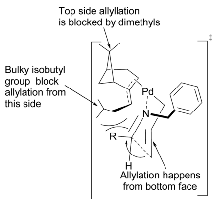
Fig. 8 Proposed transition state of (–)- \beta -pinene-based \pi -allylpalladium mediated allylation of imine.
