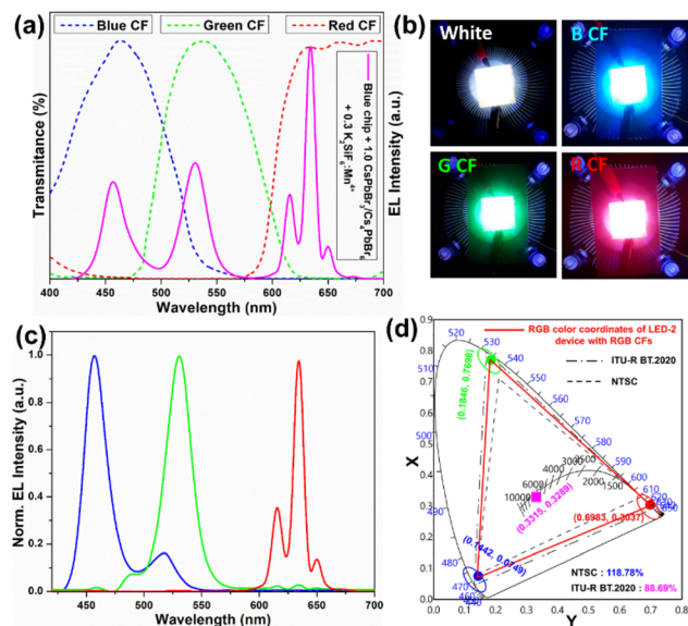
Fig. 10 (a) The transmittance spectra of commercial RGB color filters and unfiltered EL spectrum of a white-light emitting LED-2 device ( \text{K}_2\text{SiF}_6\text{:Mn}^{4+} : \text{CsPbBr}_3/\text{Cs}_4\text{PbBr}_6 in 0.3 : 1 wt% ratio), (b) photographs of an unfiltered white-light emitting LED-2 device without CFs and with RGB CFs, (c) filtered RGB EL spectra from white-light emitting LED-2 device (normalized) and (d) CIE color coordinates of filtered RGB EL spectra from a white-light emitting LED-2 device and comparison of the wide color gamut of blue chip + green-emitting \text{CsPbBr}_3/\text{Cs}_4\text{PbBr}_6 + red-emitting \text{K}_2\text{SiF}_6\text{:Mn}^{4+} indicated with NTSC standard triangle (---), and ITU-R BT.2020 triangle (---).
