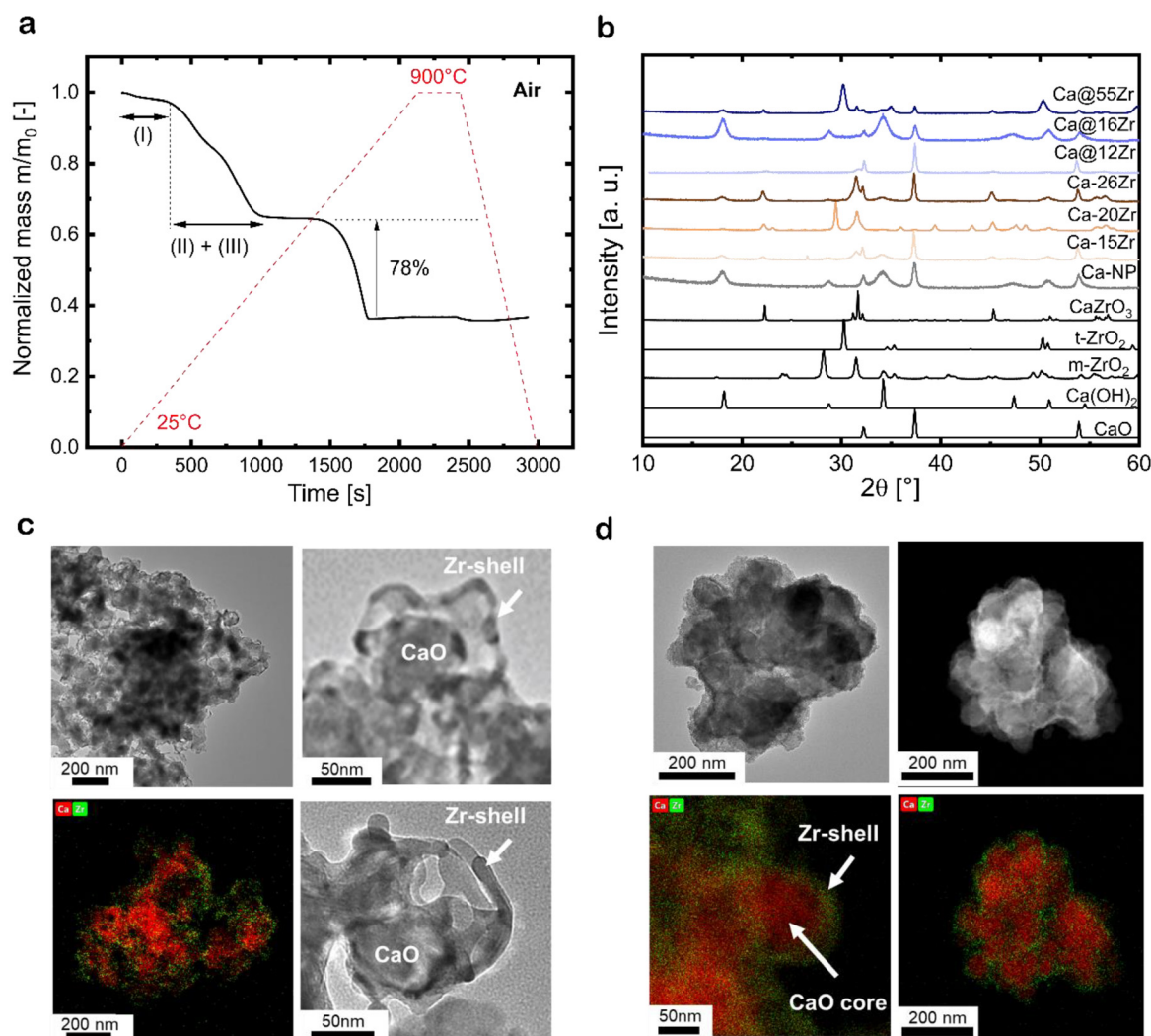
Fig. 3 (a) Weight loss of \text{CaCO}_3 nanoparticles containing a carbonaceous template coating during calcination in air (heating ramp of 25^\circ\text{C min}^{-1} up to 900^\circ\text{C} ), (b) XRD patterns of calcined zirconia-stabilized sorbents after template removal; TEM micrographs and EDX-TEM elemental maps for Ca and Zr for (c) a zirconia-stabilized, yolk-shell structured sorbent (Ca@12Zr) and (d) a zirconia-stabilized, core-shell-structured sorbent (Ca-26Zr).
