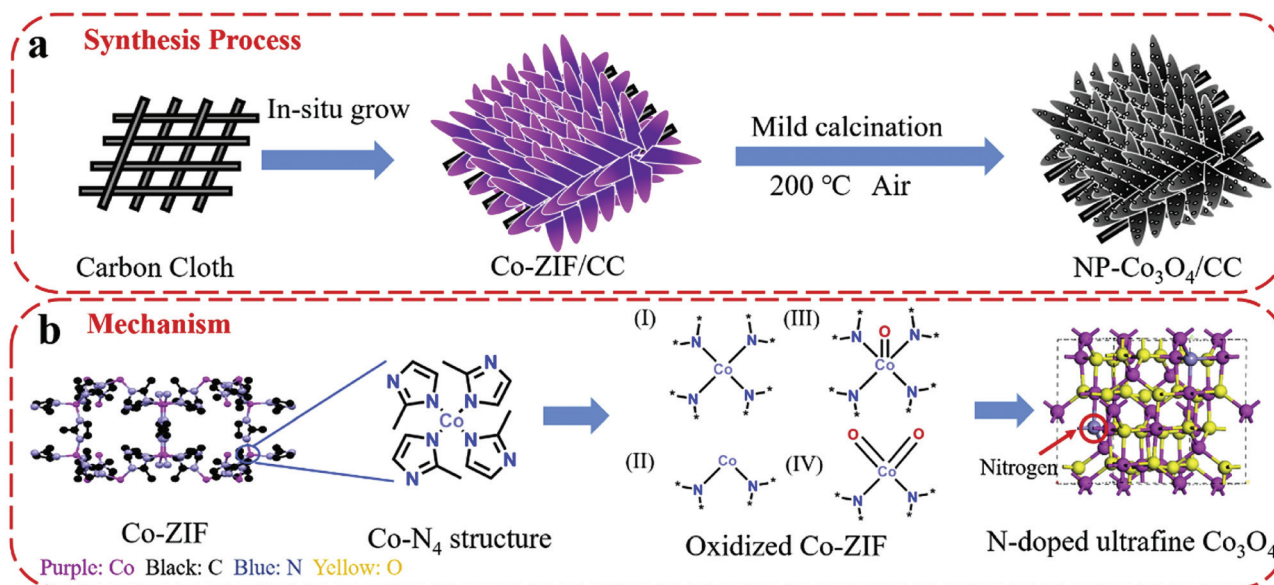
Fig. 14 Schematic demonstration of (a) the fabrication process of NP-Co 3 O 4 /CC and (b) the proposed mechanism of nitrogen doping in cobalt oxide lattices. Reproduced from ref. 282 with permission from Elsevier B.V.
