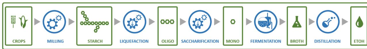
Fig. 2 Schematic representation of the steps involved in a typical process for the production of bioethanol from a first generation feedstock: corn starch.
