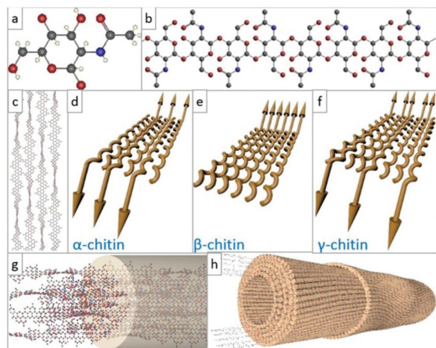
Fig. 1 The structure and configuration of chitin. (a and b) Ball-and-stick model of the dGlcNAc monomer, where red is oxygen, blue is nitrogen, and gray is carbon atom; (c) schematic diagram of chitin molecular chain arrangement; (d–f) schematic diagrams of the molecular chain orientations in the polymorphic configurations of different types of chitin; (g and h) molecular chain packaging diagram and nanofiber packaging diagram in chitin nanofibers. 54 Copyright 2021 Elsevier Ltd.
