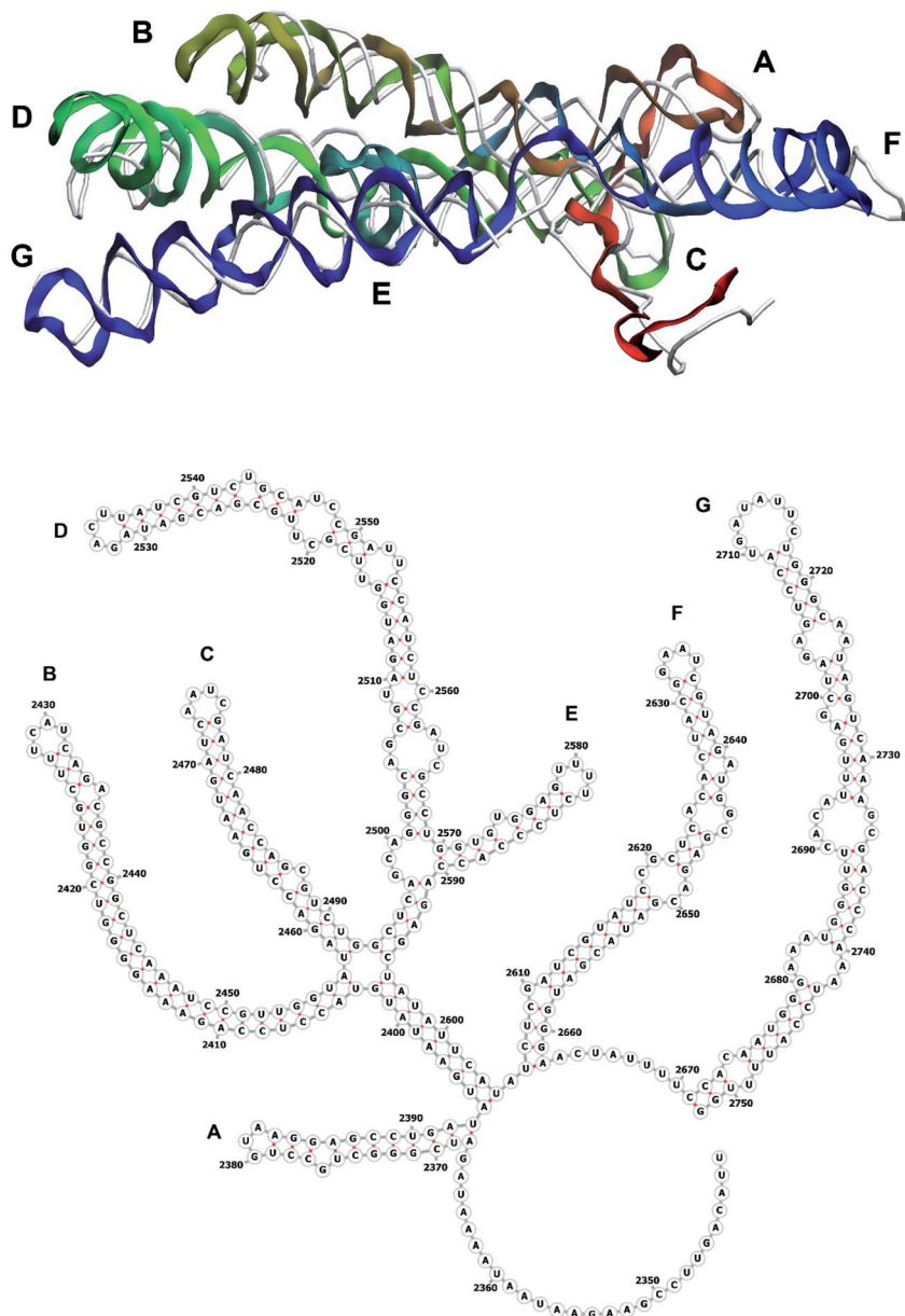
Fig. 10 Segment 2341–2752 of the reconstructed genome model (red to green to blue), placed over the cryo-EM backbone (white), and its secondary structure.
