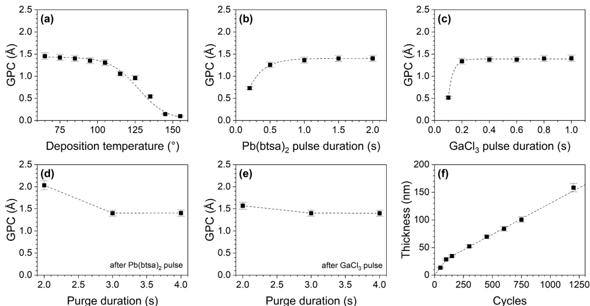
Fig. 2 Growth per cycle (GPC) of \text{PbCl}_2 on silicon as a function of (a) deposition temperature, (b) \text{Pb(btsa)}_2 pulse duration, (c) \text{GaCl}_3 pulse duration, (d) purge duration after \text{Pb(btsa)}_2 pulse and (e) purge duration after \text{GaCl}_3 pulse. (f) \text{PbCl}_2 film thickness as a function of deposition cycles. Unless otherwise evident the depositions were made at 85 °C, with 600 cycles of 1.5 s \text{Pb(btsa)}_2 pulse, 0.8 s \text{GaCl}_3 pulse and 3.0 s purge durations. Thicknesses were measured with ellipsometry.
