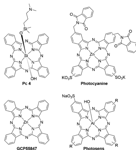
Fig. 2 Pc-based photosensitizers that have reached phased clinical trials. For photosens, R = H or SO_3Na as a mixture of di-, tri- and tetra-sulfonated compounds. Photocyanine and photosens are a statistical mixture of isomers with substituents on either \beta -position of the indicated isoindole units of the Pc.
