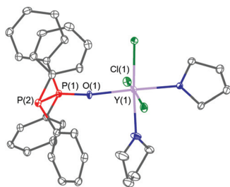
Fig. 6 Molecular structure of [\text{YCl}_3(\text{THF})_2(\text{PPO})] \cdot 0.5\text{THF} ( 2 \cdot 0.5\text{THF} ). Selected bond lengths (Å) and angles (°): \text{Y}(1) - \text{Cl}(1) 2.591(2), \text{Y}(1) - \text{Cl}(2) 2.536(1), \text{Y}(1) - \text{Cl}(3) 2.600(2), \text{Y}(1) - \text{O}(1) 2.204(4), \text{P}(1) - \text{O}(1) 1.502(4), \text{P}(1) - \text{P}(2) 2.188(2), \text{O}(1) - \text{P}(1) - \text{P}(2) 116.3(2).
