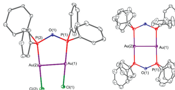
Fig. 8 (Left) molecular structure of [\text{Au}_2\text{Cl}_2(\mu_2\text{-POP})] ( 4 ) and (right) molecular structure of the cation of [\text{Au}_2(\mu_2\text{-POP})_2]^{2+} of 5 \cdot 2.3\text{DCM} . Triflate anions and DCM solvent molecules are omitted for clarity. Selected bond lengths (Å) and angles (°) for 4 : \text{Au}(1) - \text{P}(1) 2.204(1), \text{Au}(2) - \text{P}(2) 2.208(1), \text{Au}(1) - \text{Cl}(1) 2.275(1), \text{Au}(2) - \text{Cl}(2) 2.287(1), \text{Au}(1) - \text{Au}(2) 3.2055(5), \text{P}(1) - \text{O}(1) 1.615(3), \text{P}(2) - \text{O}(1) 1.616(3), \text{P}(1) - \text{O}(1) - \text{P}(2) 125.3(2). Selected bond lengths (Å) and angles (°) for 5 \cdot 2.3\text{DCM} : \text{Au}(1) - \text{P}(1) 2.312(1), \text{Au}(1) - \text{P}(2) 2.313(2), \text{Au}(2) - \text{P}(3) 2.309(1), \text{Au}(2) - \text{P}(4) 2.304(2), \text{Au}(1) - \text{Au}(2) 2.9302(7), \text{P}(1) - \text{O}(1) 1.626(4), \text{P}(2) - \text{O}(2) 1.627(4), \text{P}(3) - \text{O}(1) 1.626(4), \text{P}(4) - \text{O}(2) 1.629(4), \text{P}(1) - \text{O}(1) - \text{P}(3) 131.2(2), \text{P}(2) - \text{O}(2) - \text{P}(4) 131.7(2), \text{P}(1) - \text{Au}(1) - \text{P}(2) 179.00(6), \text{P}(3) - \text{Au}(2) - \text{P}(4) 177.52(6).
