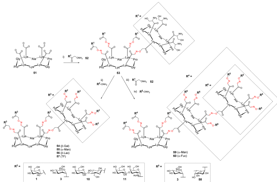
Scheme 11 Extension of the cyclodeptide valency from 16 to 64 by iterative oxime ligation. Reagents and conditions: (i) 0.1% TFA in H 2 O, 37 °C, 4 h, acetone quenching; (ii) NaIO 4 , H 2 O, r.t., 30 min then 0.1% TFA in H 2 O, 37 °C, 4 h, 65–88%; (iii) 0.1% TFA in H 2 O, 37 °C, 1 h, acetone quenching then NaIO 4 , H 2 O, r.t., 30 min, 88%; (iv) 0.1% TFA in H 2 O, 37 °C, 4 h, 83–85%.
