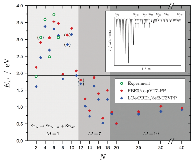
Fig. 2 Dissociation energies E D in eV for the energetically most favorable fragmentation channels of the Sn N clusters with N = 2–20, 25, 30, 40 averaged over all isomers in the given energy range. Experimental values for the incremental dissociation energies are estimated based on atomization enthalpies obtained from Knudsen cell mass spectrometry. 14 The horizontal line at 1.9 eV gives the smallest accessible single-photon energy available in our photodissociation experiment. Over the size range studied, three regions can be distinguished: dissociation under the loss of an atom (light gray), a Sn 7 (gray) and a Sn 10 fragment (dark gray). Calculated dissociation energies in parentheses point to a differing fragmentation mechanism, i.e. , loss of a Sn 2 fragment for the Sn 9 parent cluster and loss of Sn 6 fragments for the Sn 12 parent cluster. The Sn 3 experimental dissociation energy in parenthesis has been evaluated assuming a linear geometry 12 (in its lowest 1 A 1 and 3 B 2 state Sn 3 is an isoscele triangle 21 ) and has thus to be considered with care. The inset shows a typical time-of-flight mass spectrum after F 2 excimer laser photoionization (7.89 eV) of the Sn N clusters given as arbitrary intensity I in dependence of the flight time t ; the naturally low-abundant clusters Sn 13 , Sn 14 , Sn 17 and Sn 20 are highlighted by arrows.
