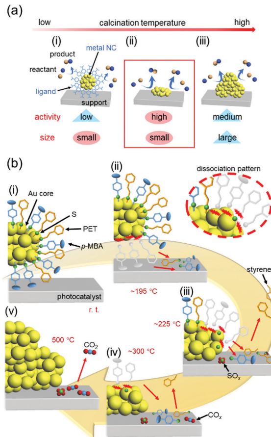
Fig. 19 (a) Schematic illustrations of the typical phenomena caused by increasing the calcination temperature in metal-oxide-supported ligand-protected metal NCs: (i) a small size is maintained but the activity is low, (ii) high activity is achieved while maintaining a small size, and (iii) the activity decreases owing to aggregation. (b) Proposed phenomenon occurring at each temperature during calcination of \text{Au}_{25}(\text{PET})_9(\text{p-MBA})_9/\text{BaLa}_4\text{Ti}_4\text{O}_{15} at (i) room temperature, (ii) ca. 195 °C, (iii) ca. 225 °C, (iv) ca. 300 °C, and (v) 500 °C. Reproduced from ref. 308. Copyright 2021 Wiley-VCH.
