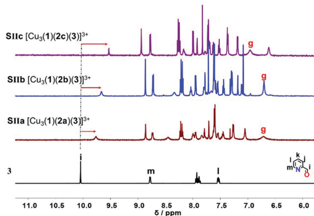
Fig. 3 Comparison of partial ^1\text{H} NMR spectra ( \text{CD}_2\text{Cl}_2 , 600 MHz, 298 K) of ligand 3 , SIla = [\text{Cu}_3(\mathbf{1})(\mathbf{2a})(\mathbf{3})]^{3+} , SIlb = [\text{Cu}_3(\mathbf{1})(\mathbf{2b})(\mathbf{3})]^{3+} , SIlc = [\text{Cu}_3(\mathbf{1})(\mathbf{2c})(\mathbf{3})]^{3+} .
