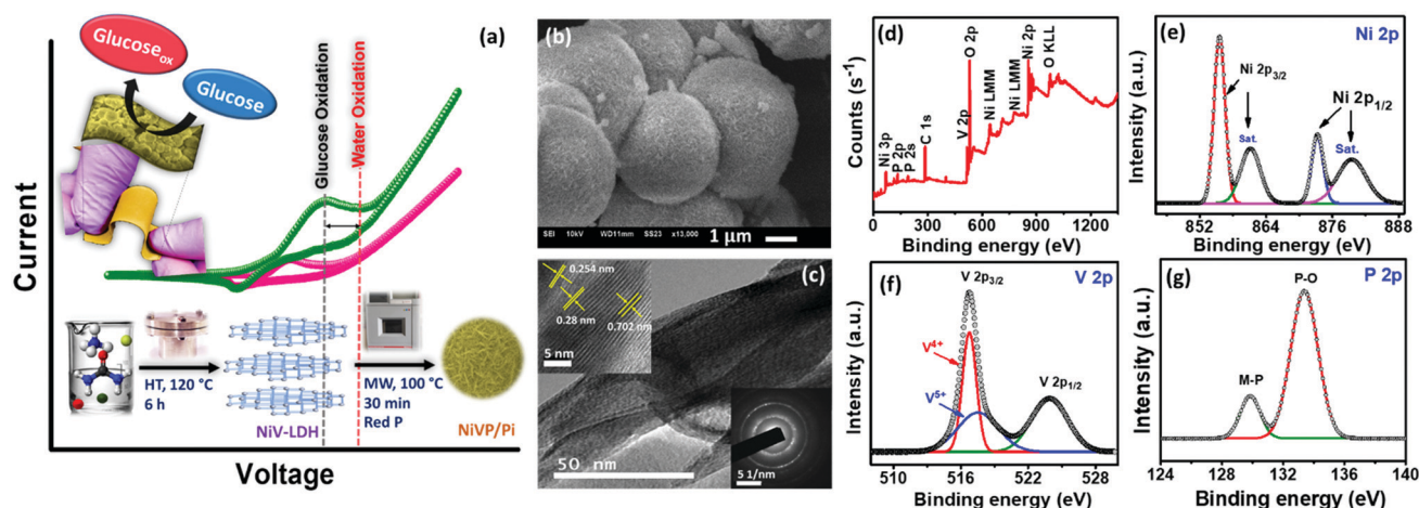
Fig. 1 (a) Schematic representation of the preparation process and glucose detection with the NiVP/Pi catalyst; (b) SEM and (c) TEM images (inset: SAED pattern, HRTEM image) of NiV(2:1)P/Pi catalyst; (d) XPS survey spectra and deconvoluted XP spectra of the: (e) Ni 2p, (f) V 2p and (g) P 2p of NiV(2:1)P/Pi catalyst.
