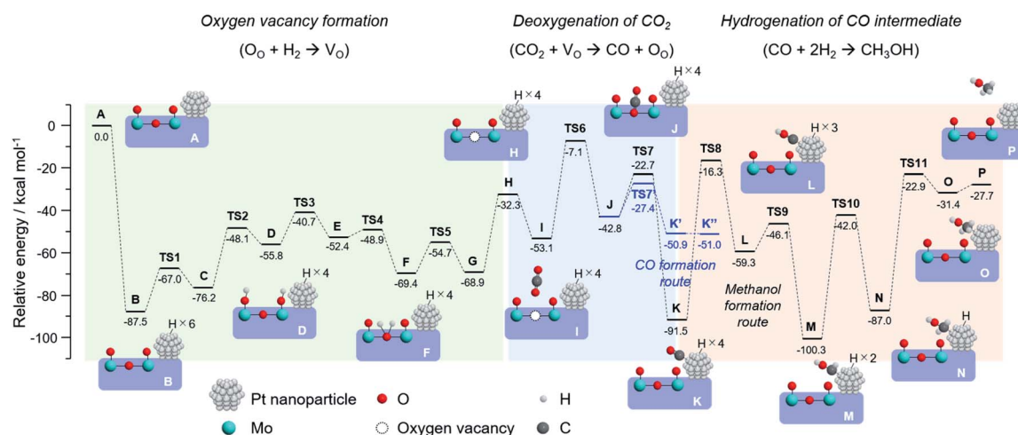
Fig. 8 Optimized reaction pathway for \text{CO}_2 hydrogenation to produce methanol, and potential energy diagram obtained by DFT calculation using \text{H}_{26}\text{Mo}_{32}\text{O}_{96}\text{-Pt}_{20} slab model and schematic illustrations of the corresponding structure models in each reaction step.
