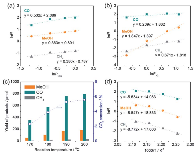
Fig. 7 (a) Double logarithm plots of reaction rate ( R ) and the partial pressure of \text{CO}_2 ( P_{\text{CO}_2} ), (b) double logarithm plots of reaction rate ( R ) and the partial pressure of \text{H}_2 ( P_{\text{H}_2} ), (c) effect of reaction temperature on catalytic performance, and (d) Arrhenius plots for the \text{Pt}/\text{H}_x\text{MoO}_{3-y}(300) catalyst. Reaction conditions: catalyst (50 mg), 1,4-dioxane (15 mL), reaction time = 2 h.
