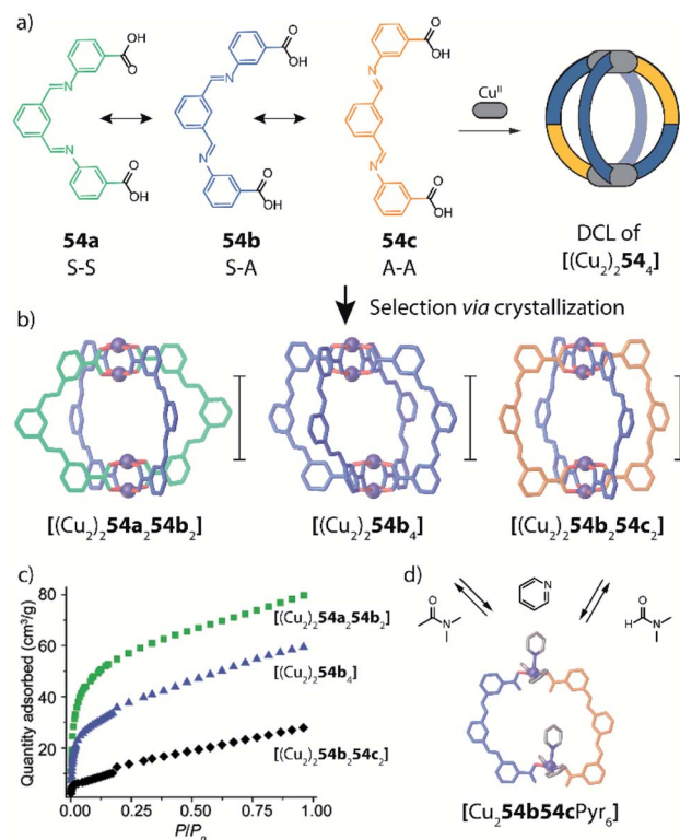
Fig. 25 (a) Ligand conformers 54a–c assemble with Cu II cations to a library of cage isomers [(Cu 2 ) 2 54 4 ]; (b) crystallization conditions allow selection of specific conformers which (c) show different CO 2 uptake characteristics and can be reversibly converted into (d) dinuclear rings by pyridine addition.
