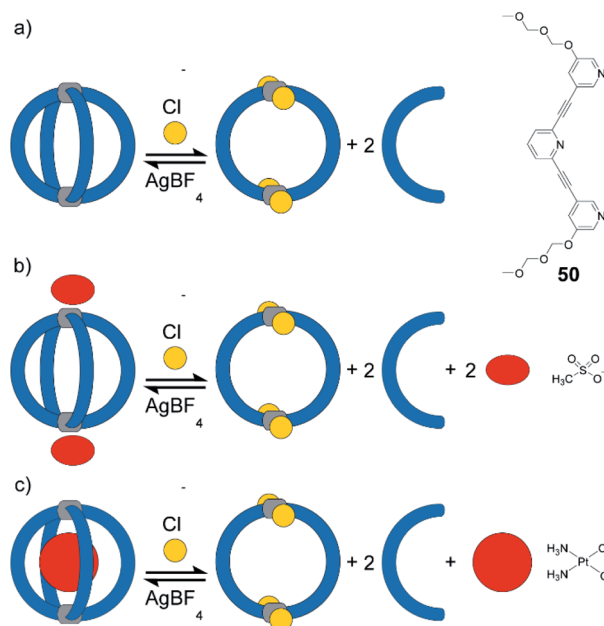
Fig. 21 (a) Reversible switch between [\text{Pd}_250_4] and [\text{Pd}_250_4\text{Cl}_4] in acetonitrile or DMF upon addition/sequestration of chloride; (b) mesylate guest binds exohedrally to [\text{Pd}_250_4] and is released upon addition of chloride; (c) cis-platin binds in the cavity of [\text{Pd}_250_4] . Formation of the ring releases the guest.
