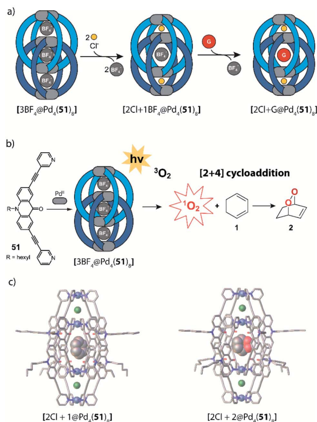
Fig. 22 (a) Chloride-triggered uptake of neutral guests by a coordination cage [\text{Pd}_451_8] following an allosteric mechanism; (b) both [3\text{BF}_4@ \text{Pd}_451_8] and [2\text{Cl} + 1@ \text{Pd}_451_8] act as photosensitizers for singlet oxygen generation. Activated oxygen adds in a [2 + 4] cycloaddition to the substrate in the cavity and surrounding solution; (c) crystal structures of [2\text{Cl} + 1@ \text{Pd}_451_8] and [2\text{Cl} + 2@ \text{Pd}_451_8] .
