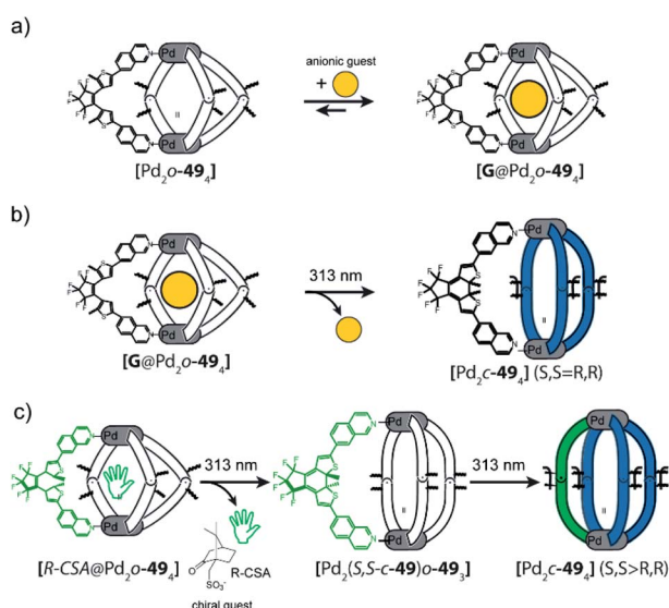
Fig. 20 (a) Binding of anionic guests in flexible DTE cage [\text{Pd}_2\text{O-49}] , (b) irradiation at 313 nm leads to closure of all photoswitches and generation of rigid [\text{Pd}_2\text{c-49}] which causes guest ejection—irradiation at 617 nm reverses this process, (c) chiral guest R -camphor sulfonate transfers chirality to the first ligand that is switched from the open to the closed form. After this the guest is released, the other three ligands switch without stereochemical control.
