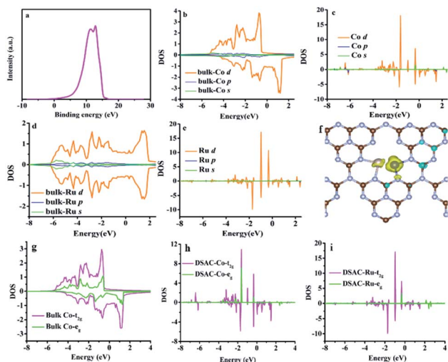
Fig. 4 UPS and PDOS results. (a) UPS spectrum. Calculated s, p, and d-orbitals over (b) Co bulk, (c) Co in RuCo DSAC, (d) Ru bulk and (e) Ru in RuCo DSAC. (f) Spin density of RuCo DSAC. (g and h) t_{2g} and e_g for (g) Co bulk, (h) Co over RuCo DSAC and (i) Ru over RuCo DSAC.
