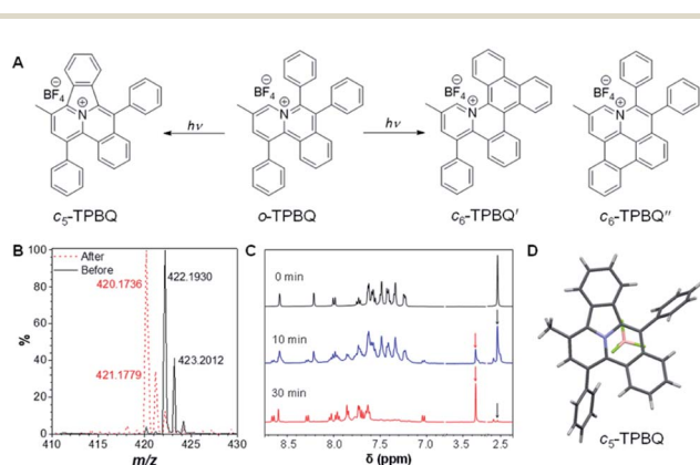
Fig. 2 (A) Possible photogenerated products. (B) High-resolution mass spectra of o -TPBQ before and after UV irradiation from a hand-held UV lamp in DMSO solution. (C) 1 H NMR spectrum of o -TPBQ under at different irradiation times. (D) Obtained single crystal structure of the photocyclized product (note: c_5 -TPBQ, instead of c_6 -TPBQ or c_6 -TPBQ', was generated in the photoreaction).
