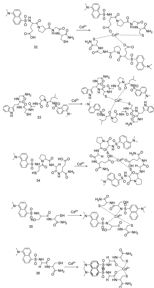
Fig. 12 The probes structure reported by P. Wang's team and proposed binding mode with Cd 2+ .
