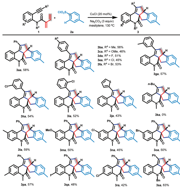
Scheme 3 Variations of the dienyynes ( 1 ). Reaction conditions: 1a (0.2 mmol), 2 (0.4 mmol), CuCl (20 mol%), Na 2 CO 3 (3 equiv.), and mesitylene (2 mL) at 130 °C under a N 2 atmosphere for 12 h; d.r. >20 : 1.
