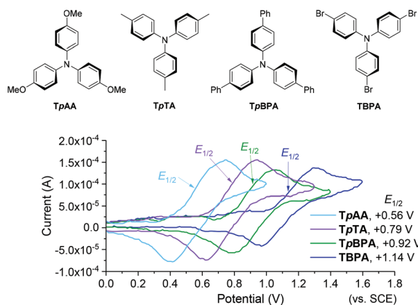
Fig. 2 First generation TPA e-PRCs (top). Cyclic voltammograms (bottom).
