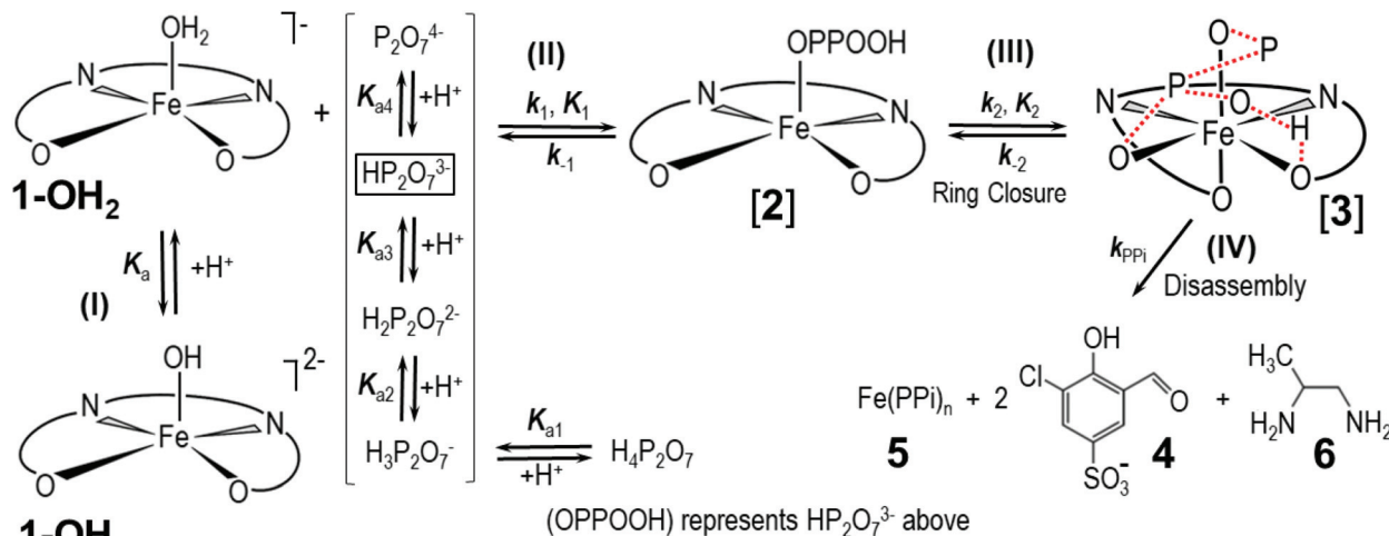
Scheme 1 Simplified reaction scheme for the disassembly as studied kinetically, with reactant species 1-OH 2 and 1-OH (interrelated by the acid dissociation constant K_a , and with [\text{PPI}]_{\text{tot}}^{47} ). Compounds [2] and [3] are assumed reactive intermediates, 5 = final \text{Fe}(\text{PPI})_n species and 4 = 3-chloro-5-sulfosalicylaldehyde. [\text{PPI}]_{\text{tot}} = total pyrophosphate concentration, of which the parent tetra-acid exhibits four \text{p}K_a values, denoted by K_{a1} , K_{a2} , K_{a3} and K_{a4} .
