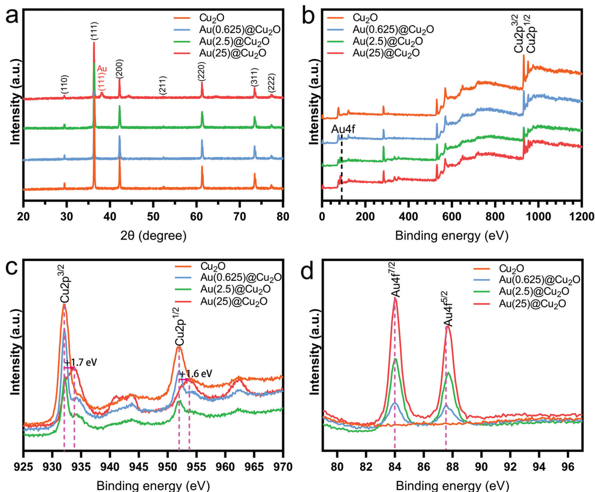
Fig. 2 The phase structure and chemical composition of \text{Cu}_2\text{O} and \text{Au}@\text{Cu}_2\text{O} nanocubes. (a) XRD patterns. (b) XPS spectra, with the survey scan ranging from 0 to 1200 eV. (c) XPS spectrum survey of the Cu 2p band. (d) XPS spectrum survey of the Au 4f band.
