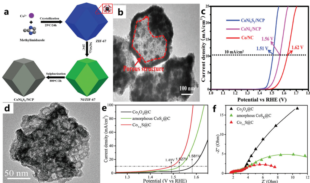
Fig. 19 (a) Schematic diagram for the fabrication of CoNiₓSᵧ/NCP. (b) TEM image of CoNiₓSᵧ/NCP. (c) Polarization curves of Co/NC, CoNiₓ/NCP, and CoNiₓSᵧ/NCP in 1 M KOH solution (scan rate: 10 mV s -1 ). 162 Copyright © 2019 Hydrogen Energy Publications LLC. Published by Elsevier Ltd. All rights reserved. (d) TEM image of Co₁₋ₓS@C. (e) LSV polarization curves of Co₃O₄@C, Co₁₋ₓS@C, and amorphous CoSₓ@C. (f) EIS Nyquist plots of Co₃O₄@C, Co₁₋ₓS@C, and amorphous CoSₓ@C. 163 Copyright © 2018 Published by Elsevier B.V. on behalf of Chinese Chemical Society and Institute of Materia Medica, Chinese Academy of Medical Sciences.
