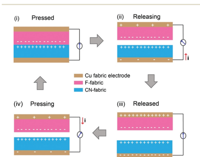
Fig. 5 Schematic diagram of the working mechanism of the N-TENG.
