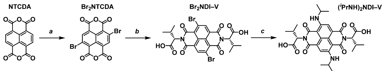
Scheme 2 The synthetic method to obtain core-functionalised blue ( i PrNH) 2 NDI-V. (a) Dibromoisocyanuric acid (2.5 eq.), H 2 SO 4 -20% SO 3 , 25 °C, 5 h, 29% yield. (b) L -Valine (2 eq.), glacial acetic acid, 120 °C, 18 h, 76% yield. (c) Isopropylamine, 25 °C, 10 days, 80% yield.
