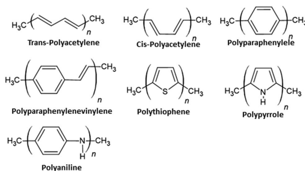
Fig. 8 Chemical structures of conductive polymers.
