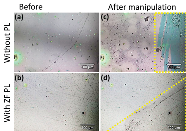
Fig. 4 Optical microscopy photographs of the surface of Tamm plasmon devices with and without PL. 4x(SB/TF)/Au and 4x(SB/TF)/Au/ZF before (a and b) and after (c and d) macroscopic damage due to manipulation. The yellow dotted lines in (c and d) mark the areas that underwent simulated mechanical manipulation.
