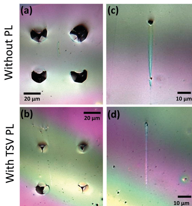
Fig. 5 Optical microscopy photographs of the surface of Tamm plasmon devices with and without PL. Array of 4 indentations up to 1000 nm depth in 4x(SC/TB)/Au (a) and 4x(SC/TB)/Au/TSV (b); scratches in the same Tamm plasmon devices, without (c) and with (d) TSV PL.
