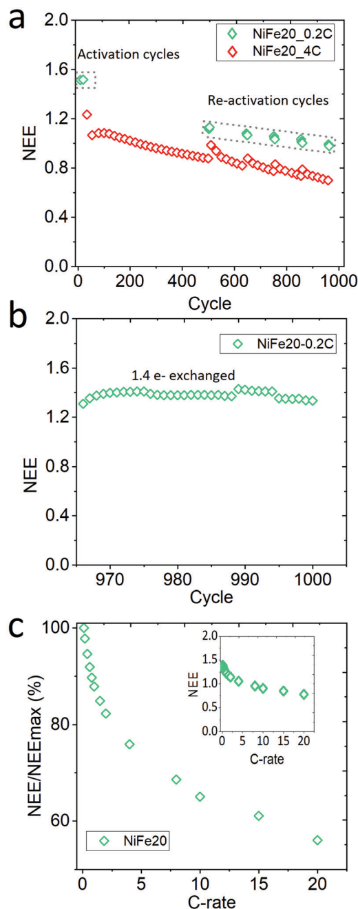
Fig. 5 Characterisation of NiFe 2 O 4 stability: (a) long-term stability test, (b) after the long-term stability test the electrode is repressed and the capacity of NiFe 2 O 4 goes back to 1.4 e - exchanged, and (c) high rate performance of the repressed electrode after the long-term stability test represented by NEE normalised by NEE at 0.1C.
