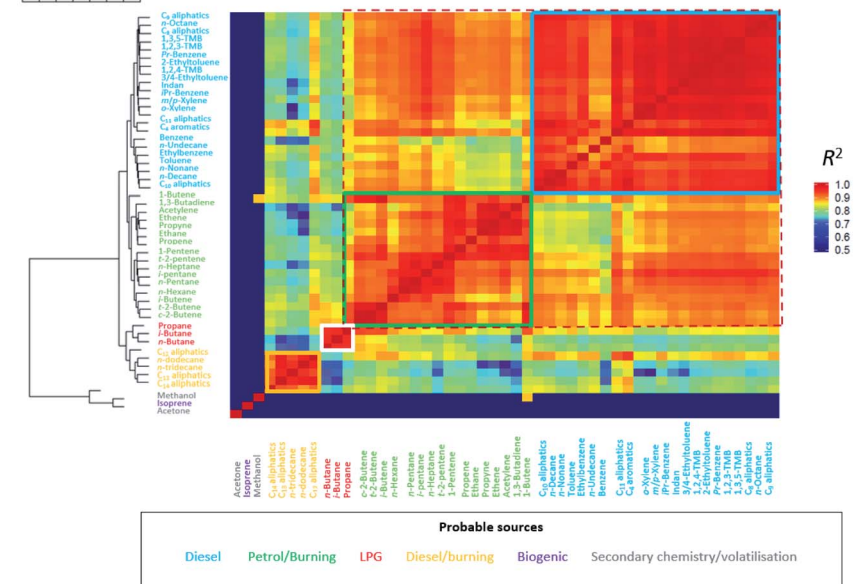
Fig. 9 Correlation and hierarchical cluster analysis of NMHC mixing ratios using a combined dataset from both pre- and post-monsoon campaigns. Light blue shaded region corresponds to hydrocarbons typically associated with diesel fuel, green region to petrol, white region to LPG and orange region to diesel/burning.
