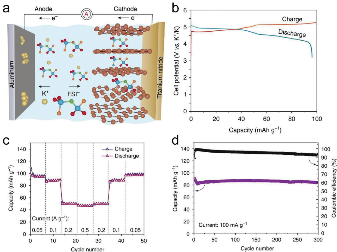
Fig. 28 (a) Schematic of the charging process in a K/C DIB. Fluorine, oxygen, sulfur, and nitrogen atoms in the \text{FSI}^- anion are shown in brown, red, blue, and green colors, respectively. (b) Typical galvanostatic voltage profile of a K/C DIB measured at a current density of 50 \text{ mA g}^{-1} . (c) Rate capability measurements and (d) cycling performance of a K/C DIB. Reproduced from ref. 167 with permission from Springer Nature.
