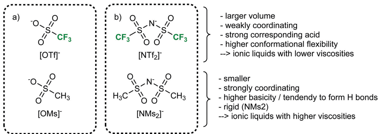
Fig. 24 Fluorinated (top row) and non-fluorinated (bottom row) anions and their typically observed behaviours. Fluorinated anions such as (a) [OTf] or [NTf_2] are often used for their beneficial physicochemical properties.
