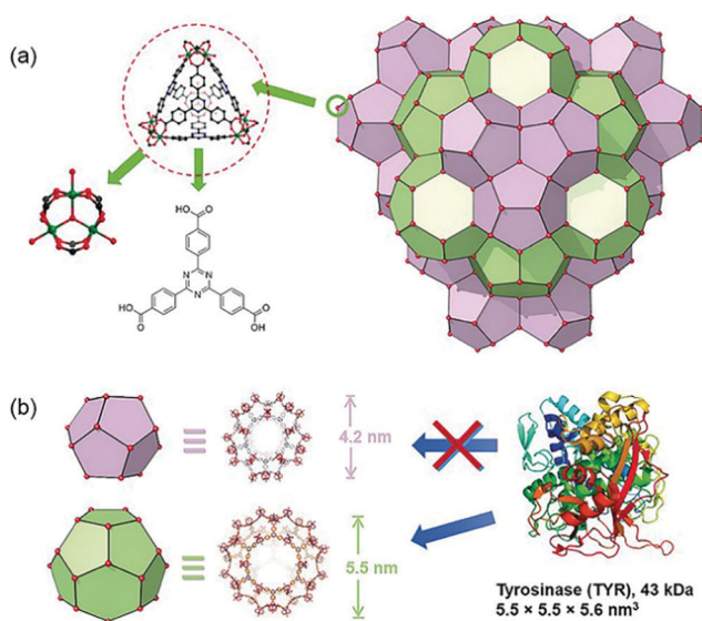
Fig. 5 The structure of NPCN-333 with two kinds of mesoporous cavities. Reprinted with permission. 69 Copyright 2018 John Wiley and sons.
