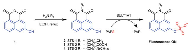
Fig. 1 Synthesis of the sulfotransferase sensors STS-1, STS-2, and STS-3 and proposed sulfurylation of the embedded 2-naphthol (shown in blue) to generate a turn-on fluorescence response. The sulfonyl group is shown in red and is transferred from the PAPS (3'-phosphoadenosine-5'-phosphosulfate) cofactor to the sensor, generating the PAP (3'-phosphoadenosine-5'-phosphate) byproduct.
